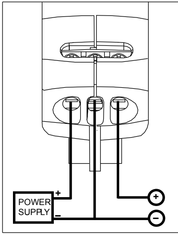
Figure 3 Voltage Output Wiring
