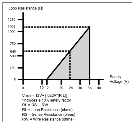
Figure 5 Load Limitations
