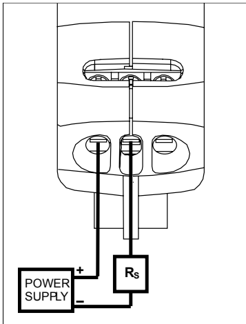
Figure 4 Current Output Wiring
