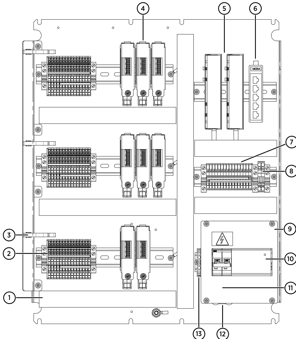
Figure 30 Main components inside CAB100B, analog channel model
