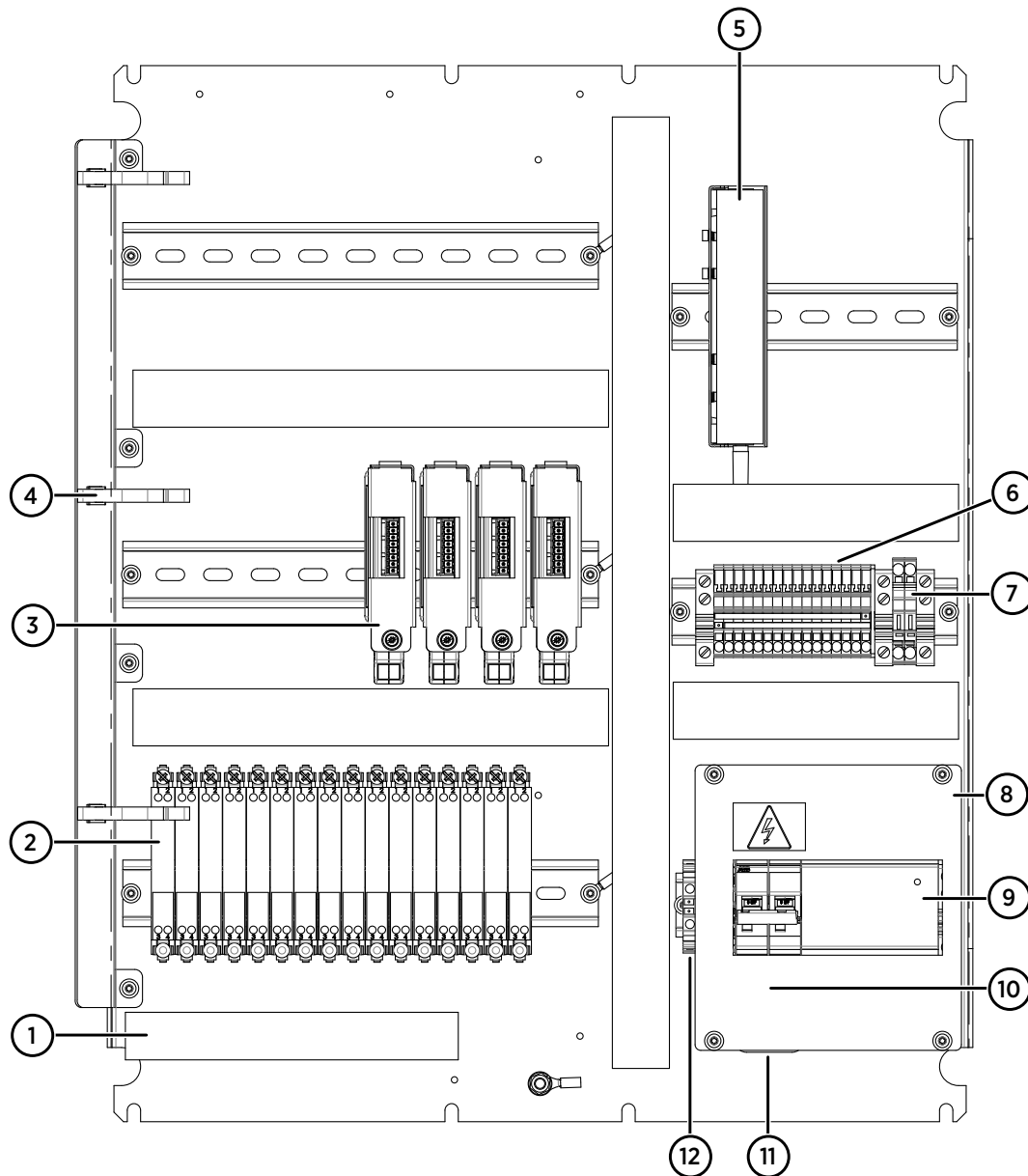
Figure 32 Main components inside CAB100B, safety barrier model
