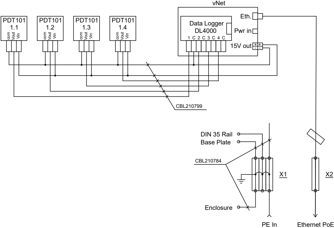
Figure 14 Wiring diagram for CAB100A PDT101 voltage model with vNet PoE
