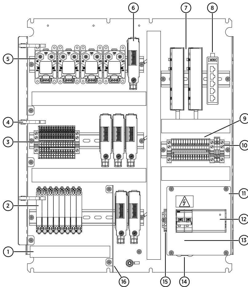
Figure 28 Main components inside CAB100B, mixed model with PDT101s, analog input channels, and safety barriers
