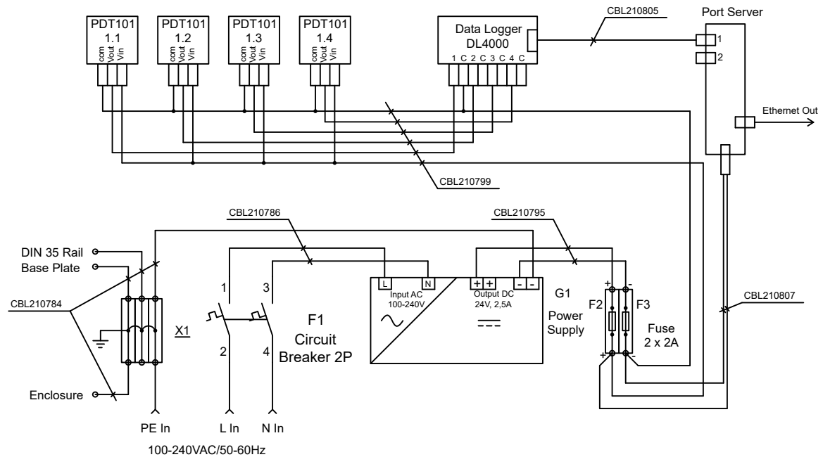
Figure 13 Wiring diagram for CAB100A PDT101 voltage model with serial port server and 24 V DC power supply
