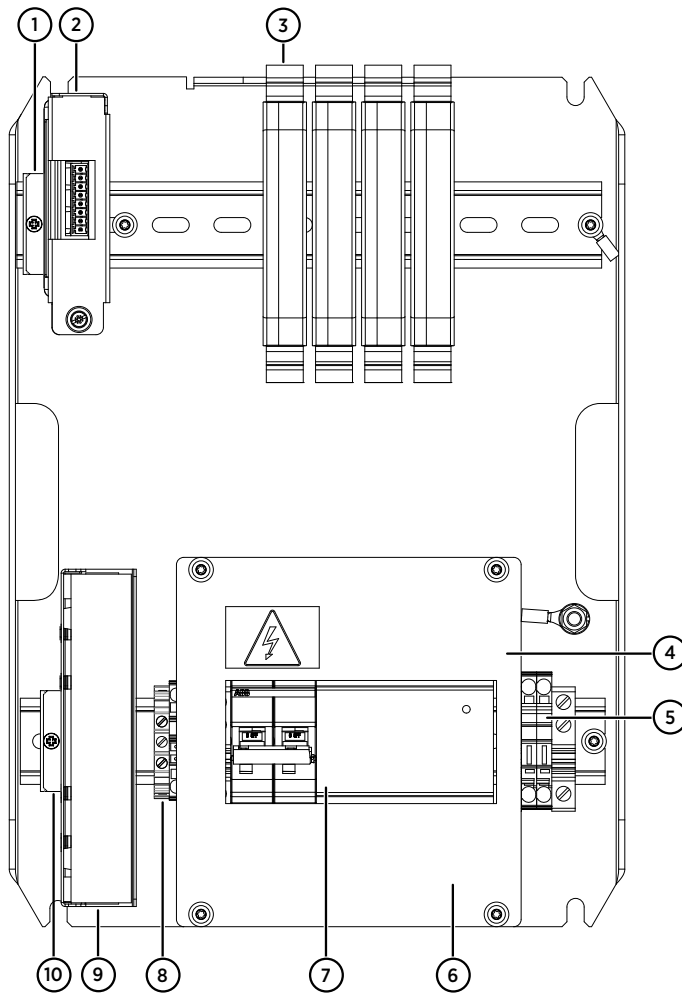
Figure 27 Main components inside CAB100A, galvanic isolator model with serial port server and 24 V DC power supply
