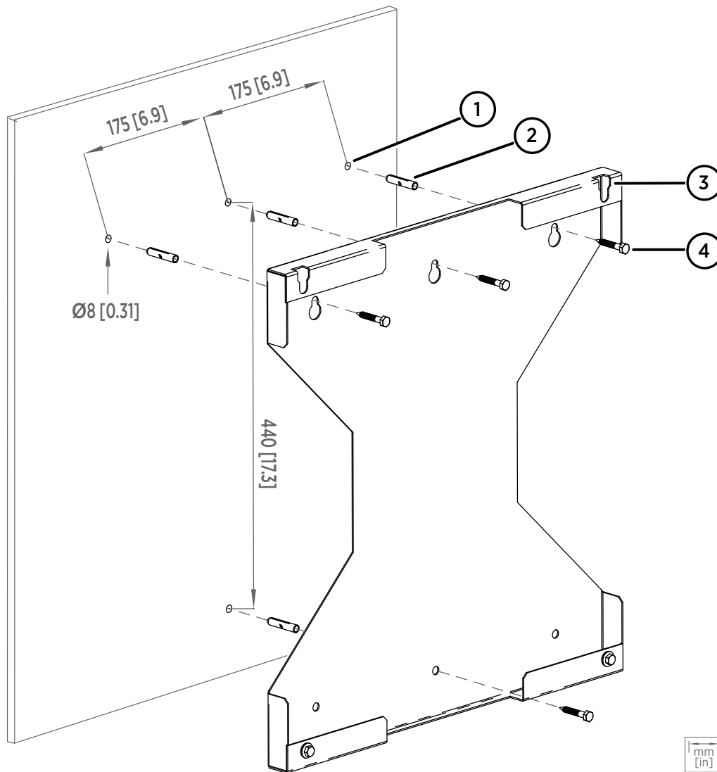
Figure 9 CAB100B wall installation accessories
