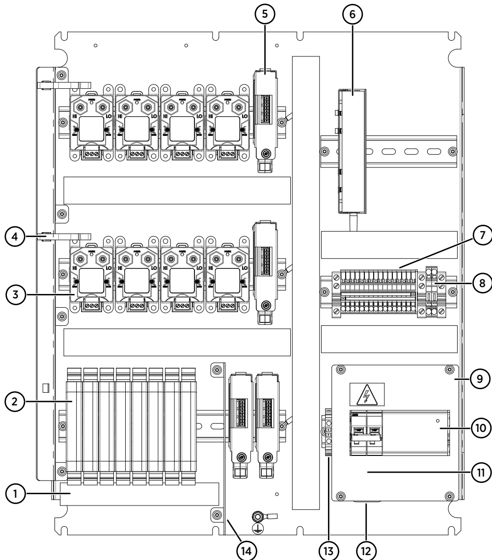
Figure 33 Main components inside CAB100B, galvanic isolator model
