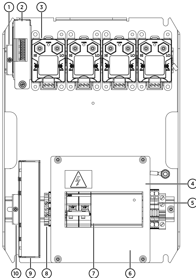
Figure 23 Main components inside CAB100A, PDT101 model with serial port server and 24 V DC power supply
