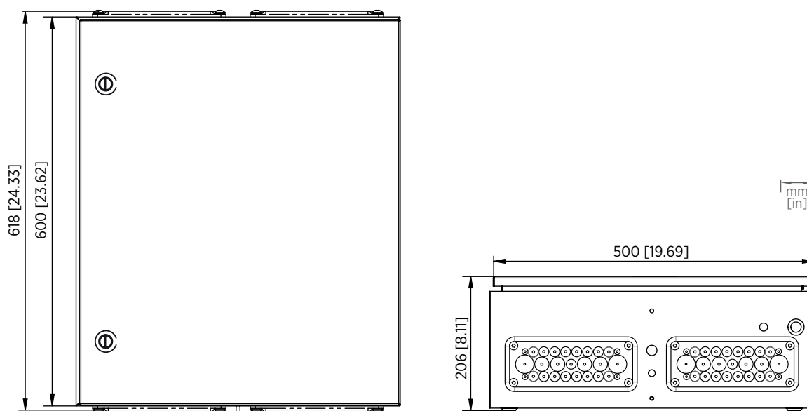
Figure 12 CAB100B enclosure dimensions
