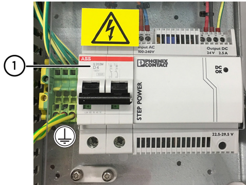
1 Circuit breaker
