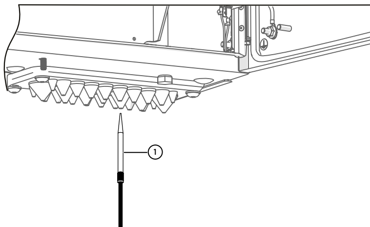
1 Pipette for leading cable through rubber flange
