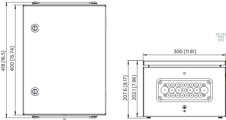
Figure 11 CAB100A enclosure dimensions
