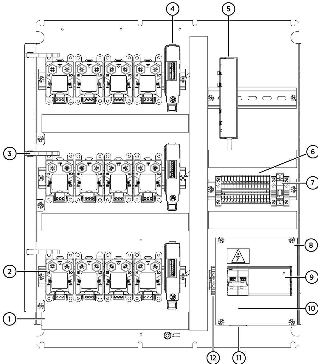
Figure 29 Main components inside CAB100B, PDT101 model
