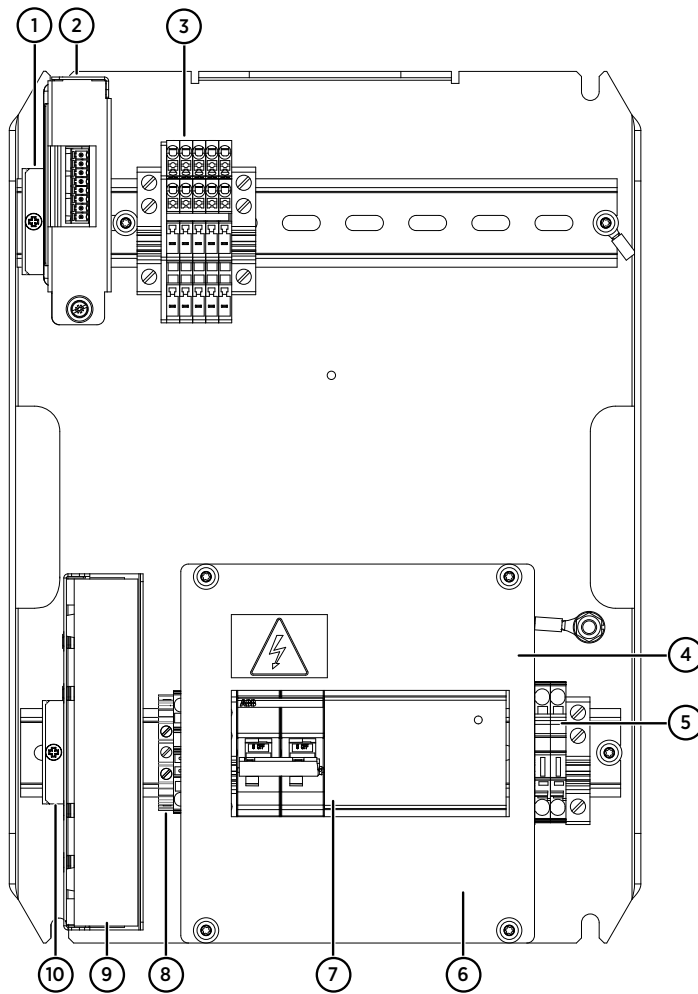
Figure 25 Main components inside CAB100A, analog channel model with serial port server and 24 V DC power supply
