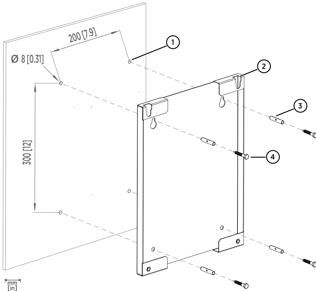
Figure 8 CAB100A wall installation accessories
