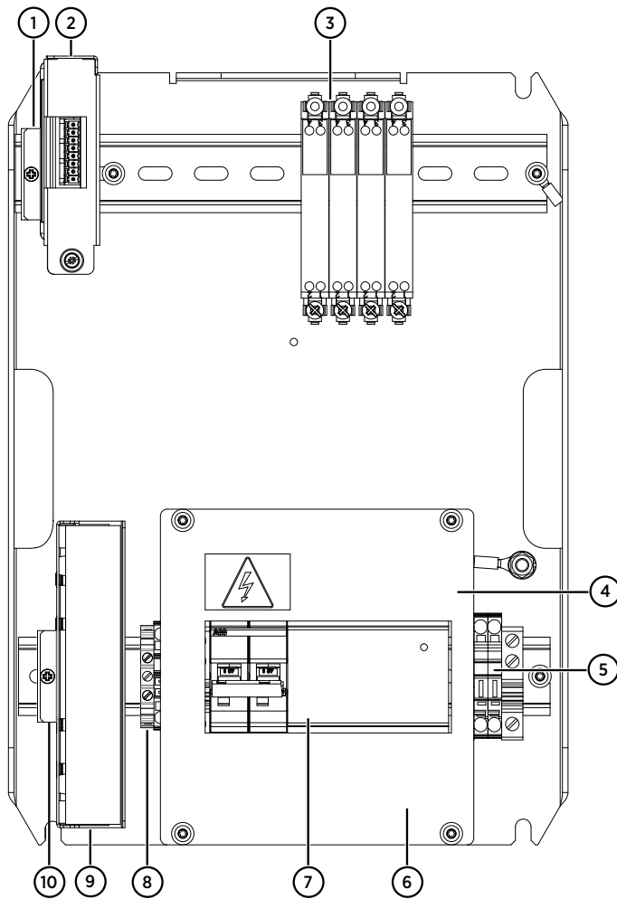
Figure 26 Main components inside CAB100A, safety barrier model with serial port server and 24 V DC power supply
