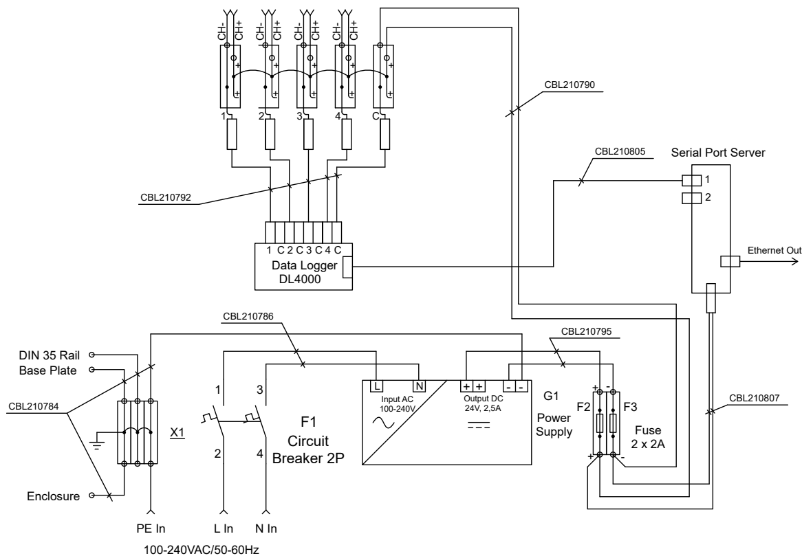
Figure 15 Wiring diagram for CAB100A analog channel model with serial port server and 24 V DC power supply
