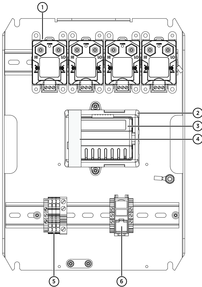
Figure 24 Main components inside CAB100A, PDT101 model with vNet PoE
