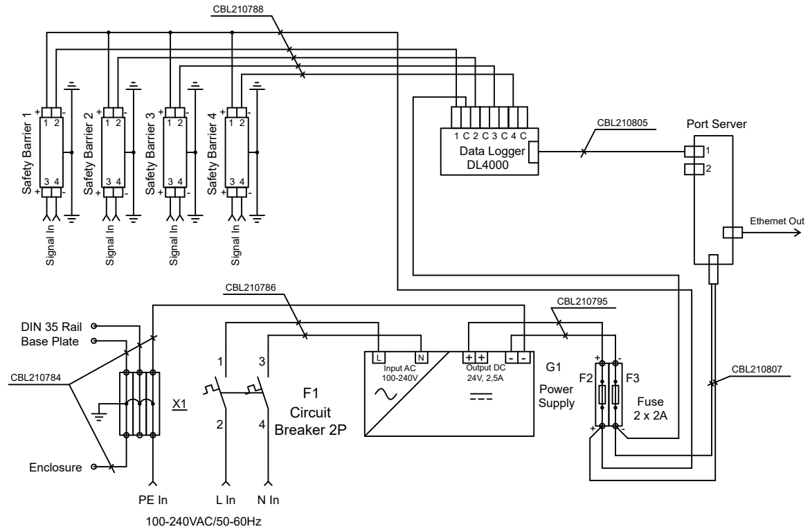
Figure 16 Wiring diagram for CAB100A safety barrier model with serial port server and 24 V DC power supply
