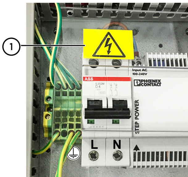
Figure 7 Risk of electric shock warning label inside the cabinet
