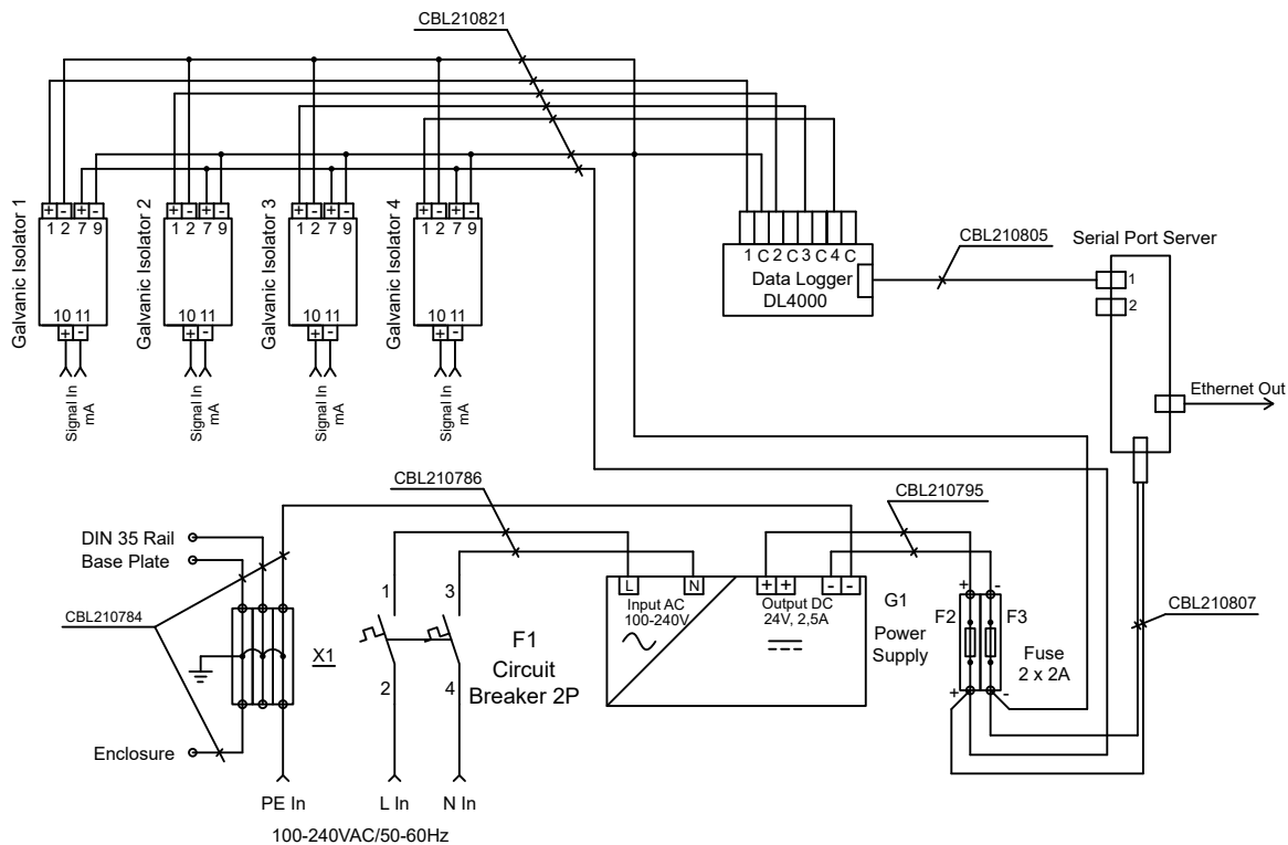
Figure 17 Wiring diagram for CAB100A galvanic isolator model with serial port server and 24 V DC power supply
