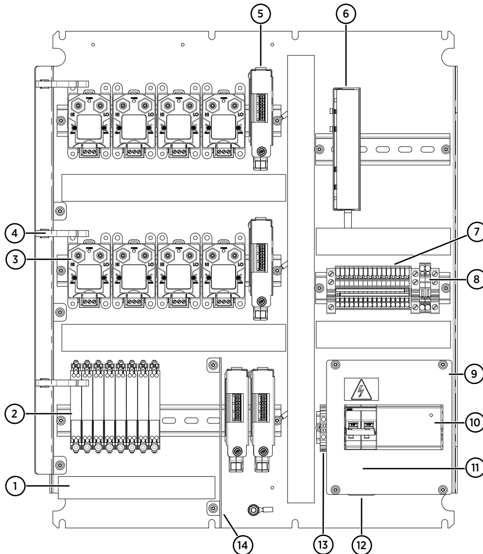
Figure 31 Main components inside CAB100B, mixed model with PDT101s and safety barriers
