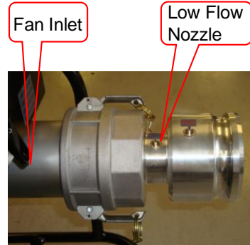
Figure 7. Positive Pressure, Low-Flow Setup
