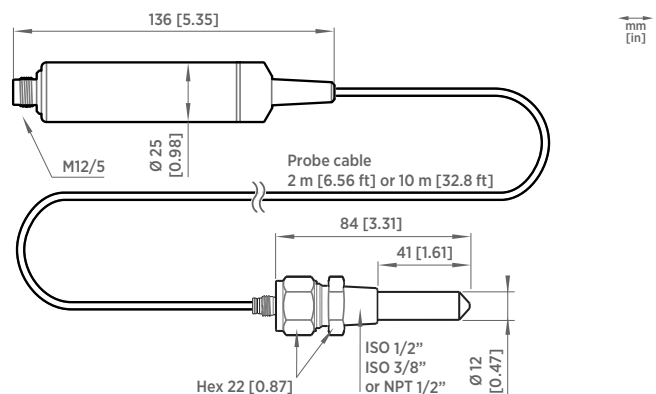
DMP7 dimensions
