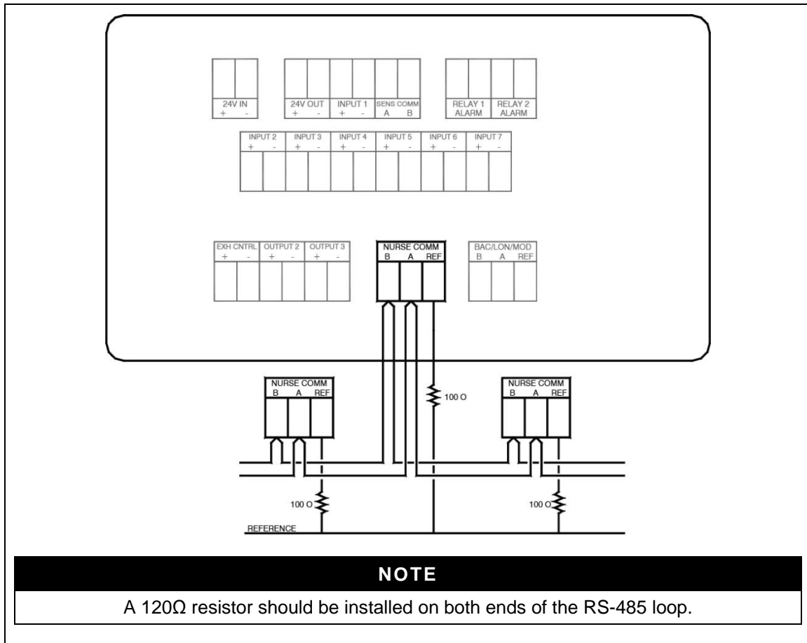
Figure 33. Optional Nurses Station Communications Wiring to Model RPM10/RPM20
