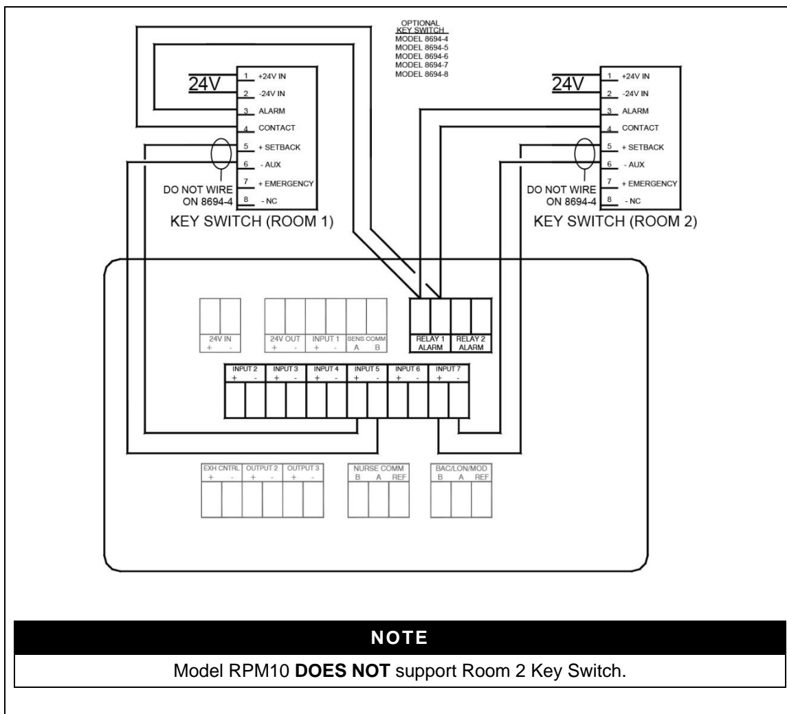
Figure 29. Optional Key Switch Wiring to Model RPM10/RPM20
