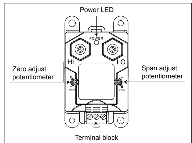
Figure 2 PDT101 Transmitter
