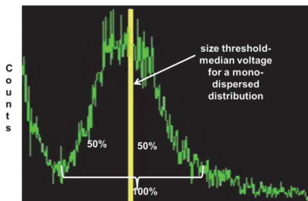
Figure 4. Determination of particle size calibration
