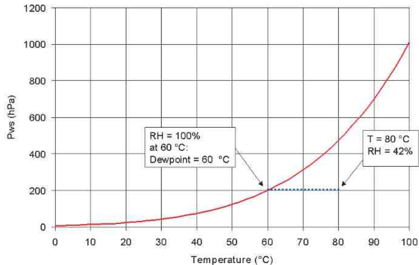
Figure 2. Dewpoint of gas at 80 ^{\circ}\text{C} and 42% RH.
