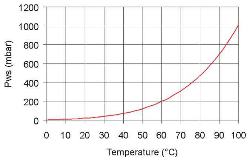
Figure 1. Water vapor saturation pressure curve
