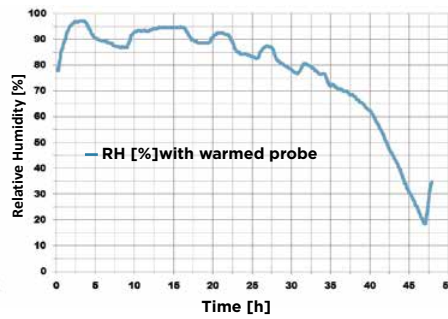
A 48-hour drying cycle with the old system (left) and the Vaisala HMT337 with warmed probe (right). The warmed-probe technology provides accurate relative-humidity readings at the beginning of the process, where the non-heated probe is saturated by condensed water.
