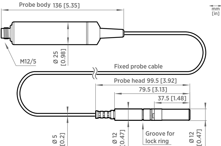
Figure 11 HMP7 probe dimensions
