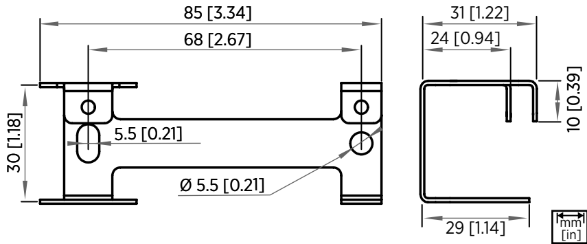
Figure 25 HPP272WALLMOUNT dimensions
