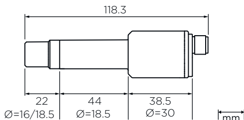
Figure 22 HPP271 dimensions
