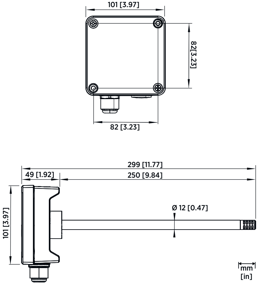
Figure 2 HMD60 Dimensions
