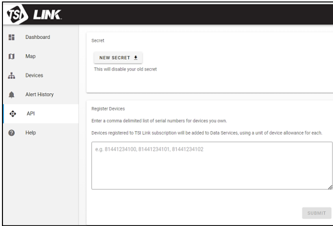
Figure 26: API menu
