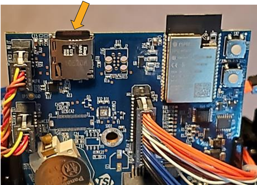
Figure 31: Location of microSD card holder
