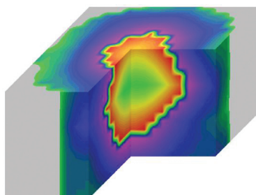
Figure 2: Cavern in the centre of a 50 liter vessel which was stirred with a Scaba 6SRGT impeller. The image shows that the cavern formed did not reach the sides of the tank or fill the complete volume of the fluid.
