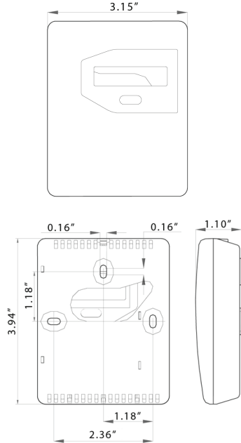
Office wall mount with optional LED display
