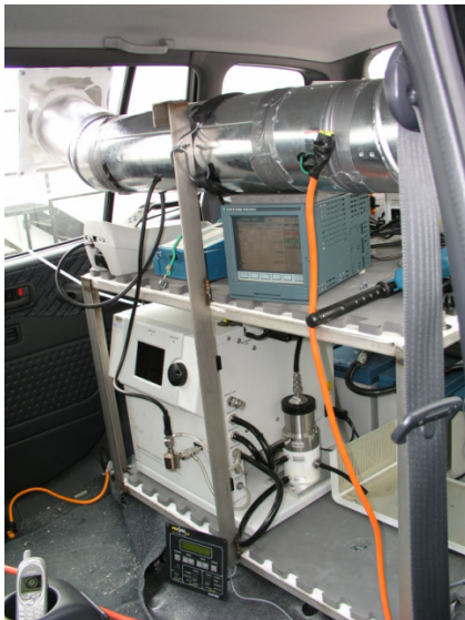
The platform, including duct work, power supplies, and computers for data logging, was jammed into the passenger and luggage compartments, leaving barely enough room for a driver and operator. Photo: Dane Westerdahl
